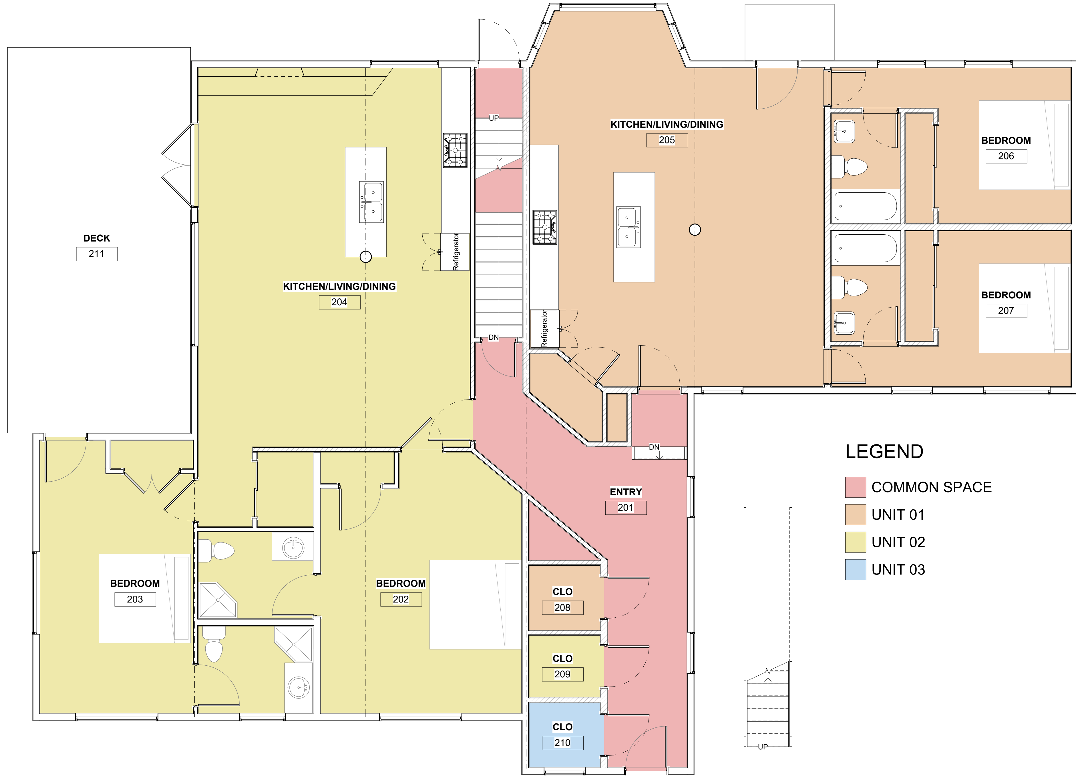
1 MAIN LEVEL - PROPOSED 1/4" = 1'-0"
